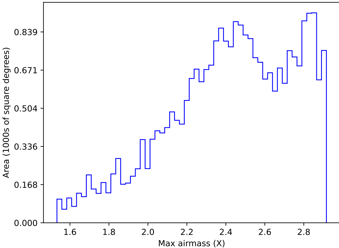
weather_cloudso0v3.4_10yrs All sky i band: Max airmass
