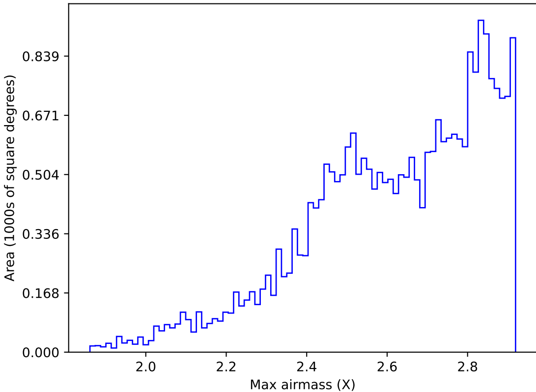
weather_cloudso0v3.4_10yrs All sky all bands: Max airmass
