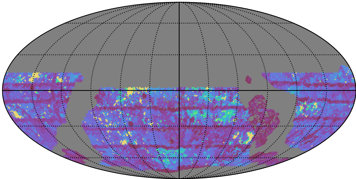
weather_cloudso0v3.4_10yrs WFD z band: Max Inter-Night Gap
