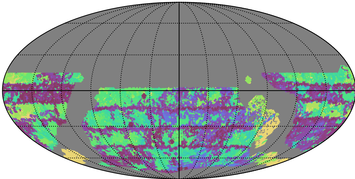
weather_cloudso0v3.4_10yrs WFD u band: Max Inter-Night Gap
