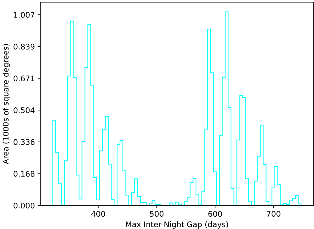
weather_cloudso0v3.4_10yrs WFD u band: Max Inter-Night Gap
