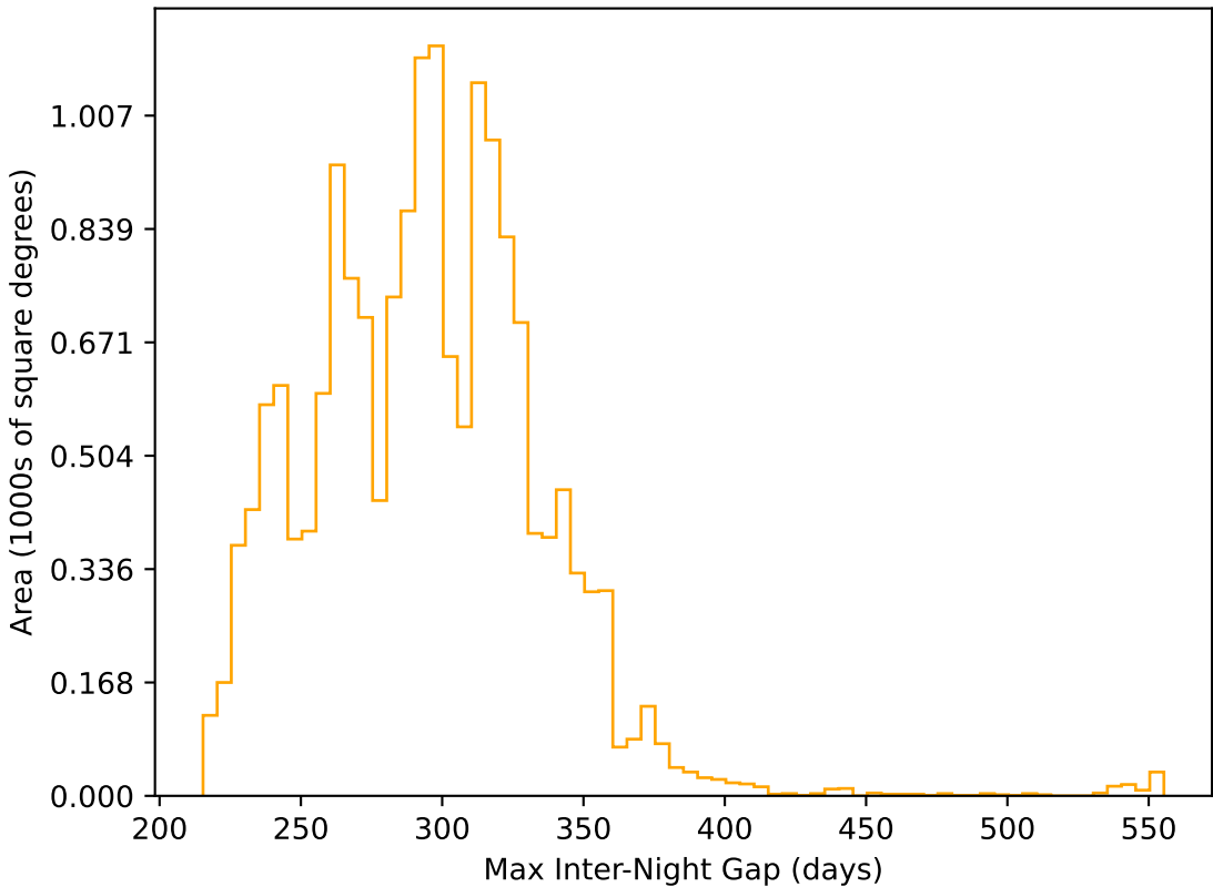
weather_cloudso0v3.4_10yrs WFD r band: Max Inter-Night Gap
