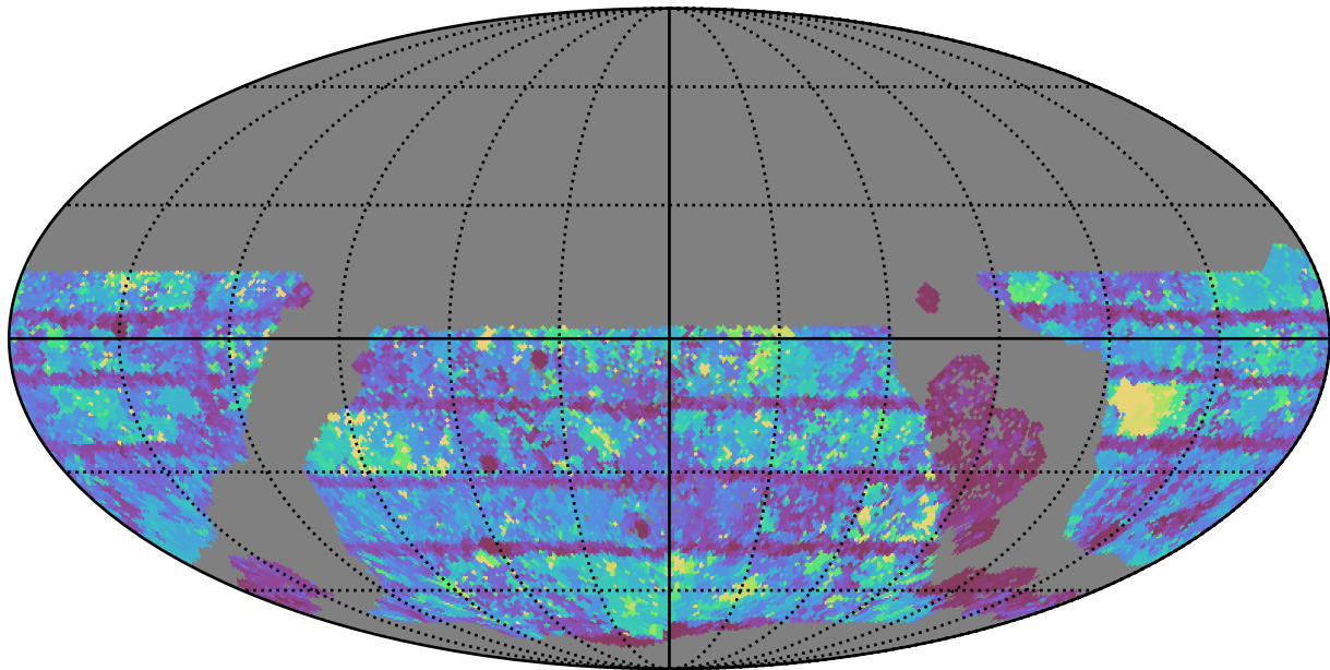
weather_cloudso0v3.4_10yrs WFD i band: Max Inter-Night Gap
