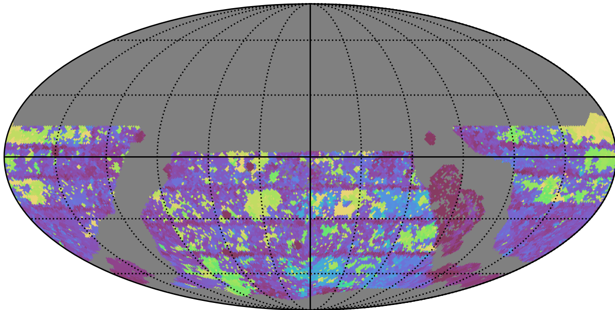
weather_cloudso0v3.4_10yrs WFD g band: Max Inter-Night Gap
