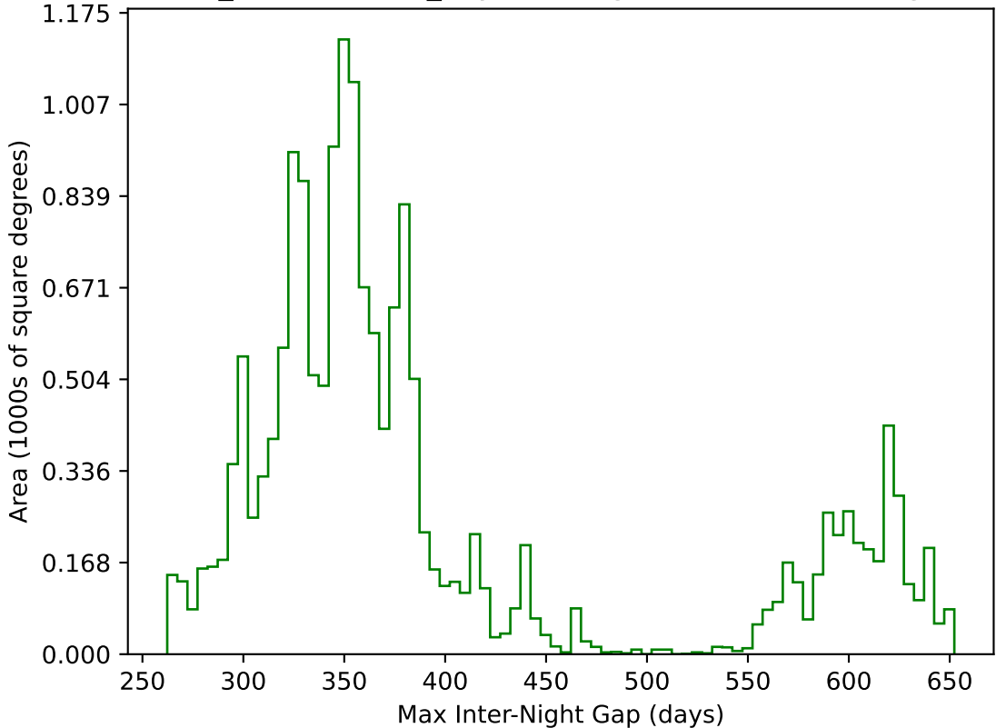
weather_cloudso0v3.4_10yrs WFD g band: Max Inter-Night Gap
