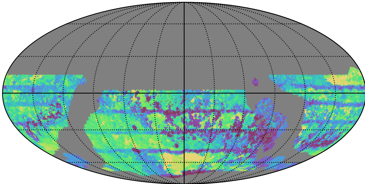
weather_cloudso0v3.4_10yrs WFD all bands: Max Inter-Night Gap
