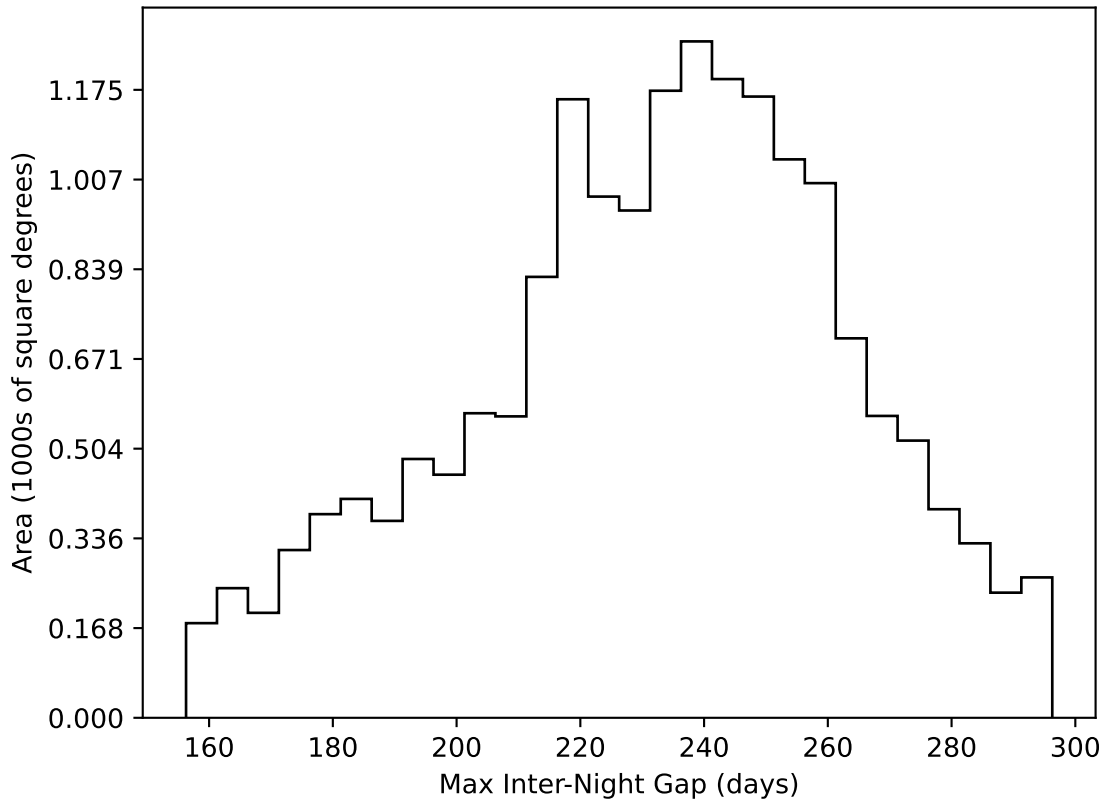
weather_cloudso0v3.4_10yrs WFD all bands: Max Inter-Night Gap
