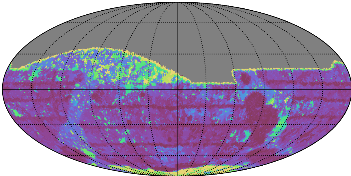
weather_cloudso0v3.4_10yrs All sky z band: Max Inter-Night Gap
