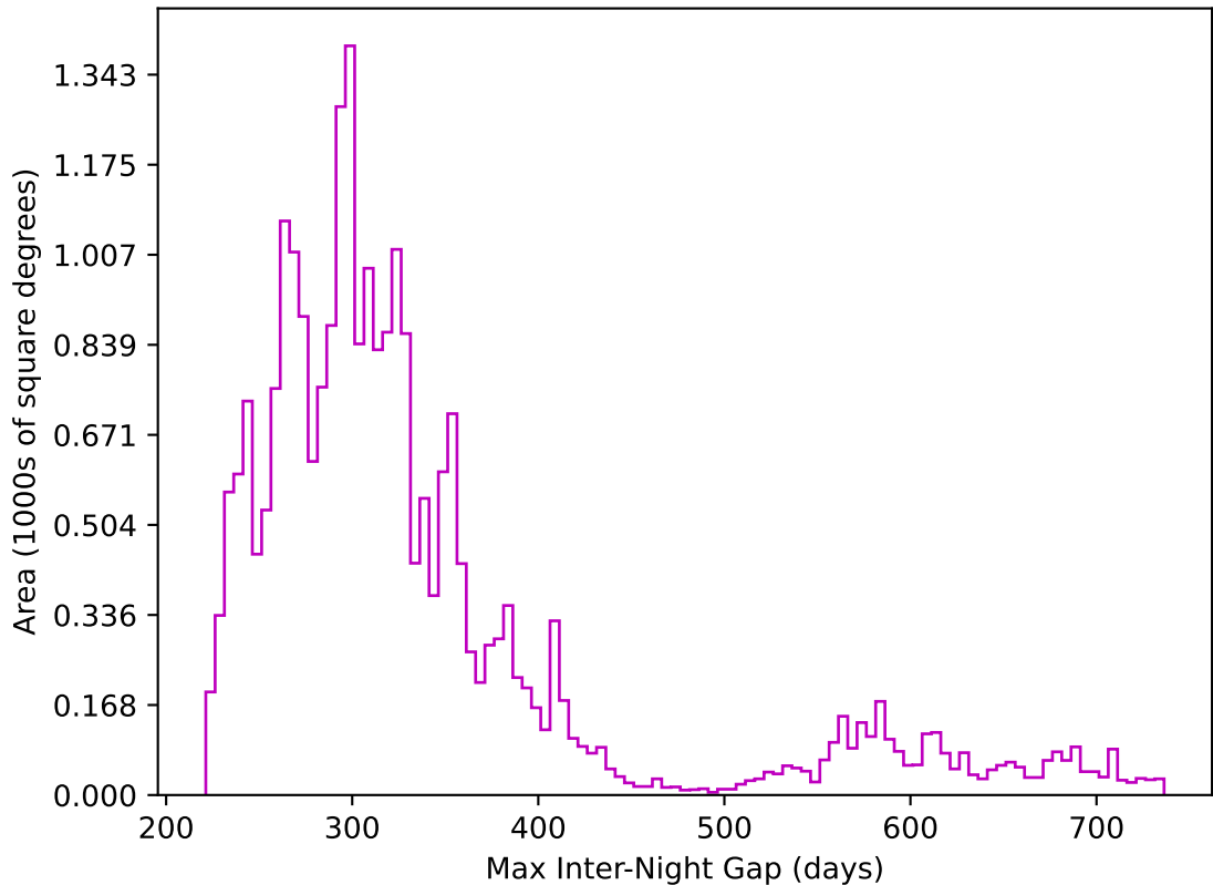
weather_cloudso0v3.4_10yrs All sky z band: Max Inter-Night Gap
