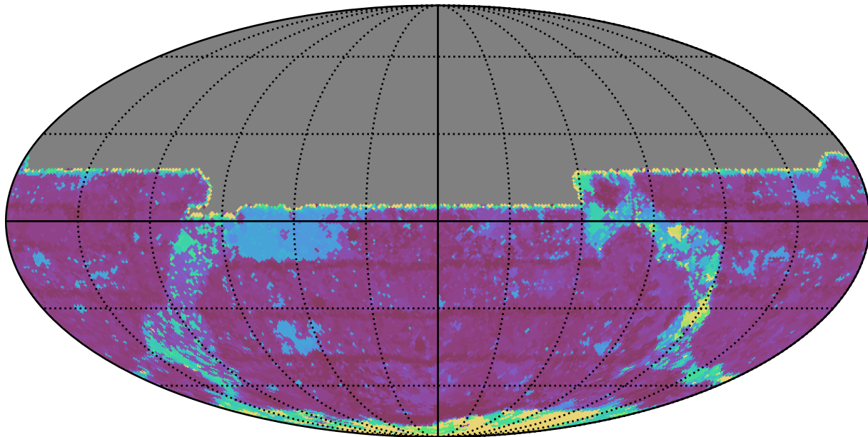
weather_cloudso0v3.4_10yrs All sky y band: Max Inter-Night Gap
