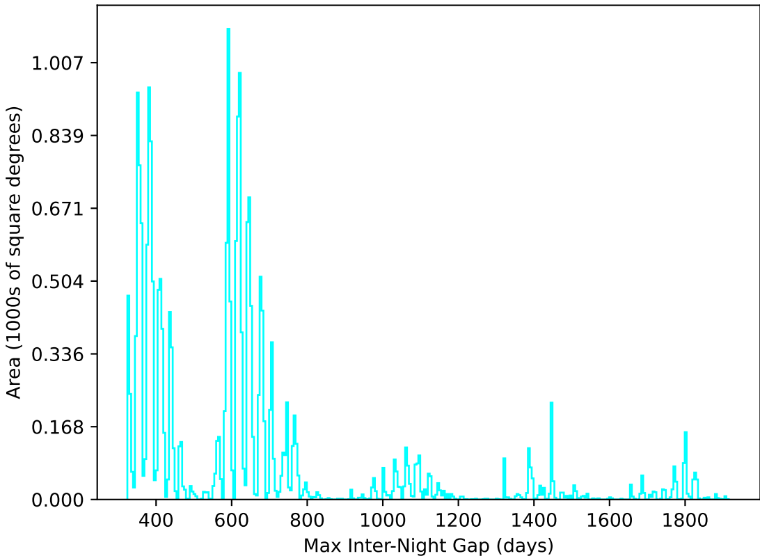
weather_cloudso0v3.4_10yrs All sky u band: Max Inter-Night Gap
