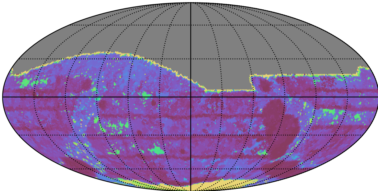
weather_cloudso0v3.4_10yrs All sky r band: Max Inter-Night Gap
