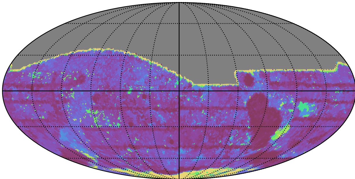
weather_cloudso0v3.4_10yrs All sky i band: Max Inter-Night Gap
