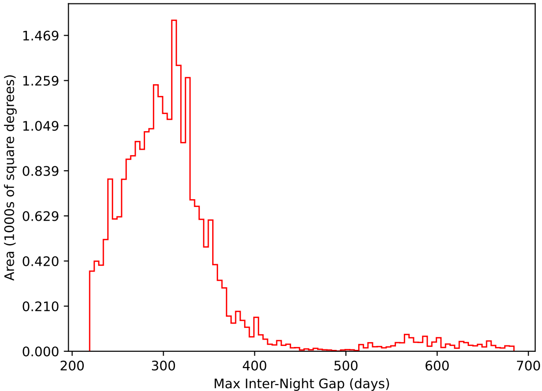
weather_cloudso0v3.4_10yrs All sky i band: Max Inter-Night Gap
