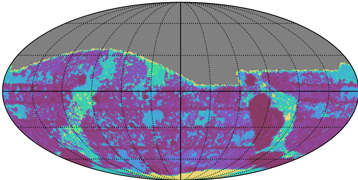
weather_cloudso0v3.4_10yrs All sky g band: Max Inter-Night Gap
