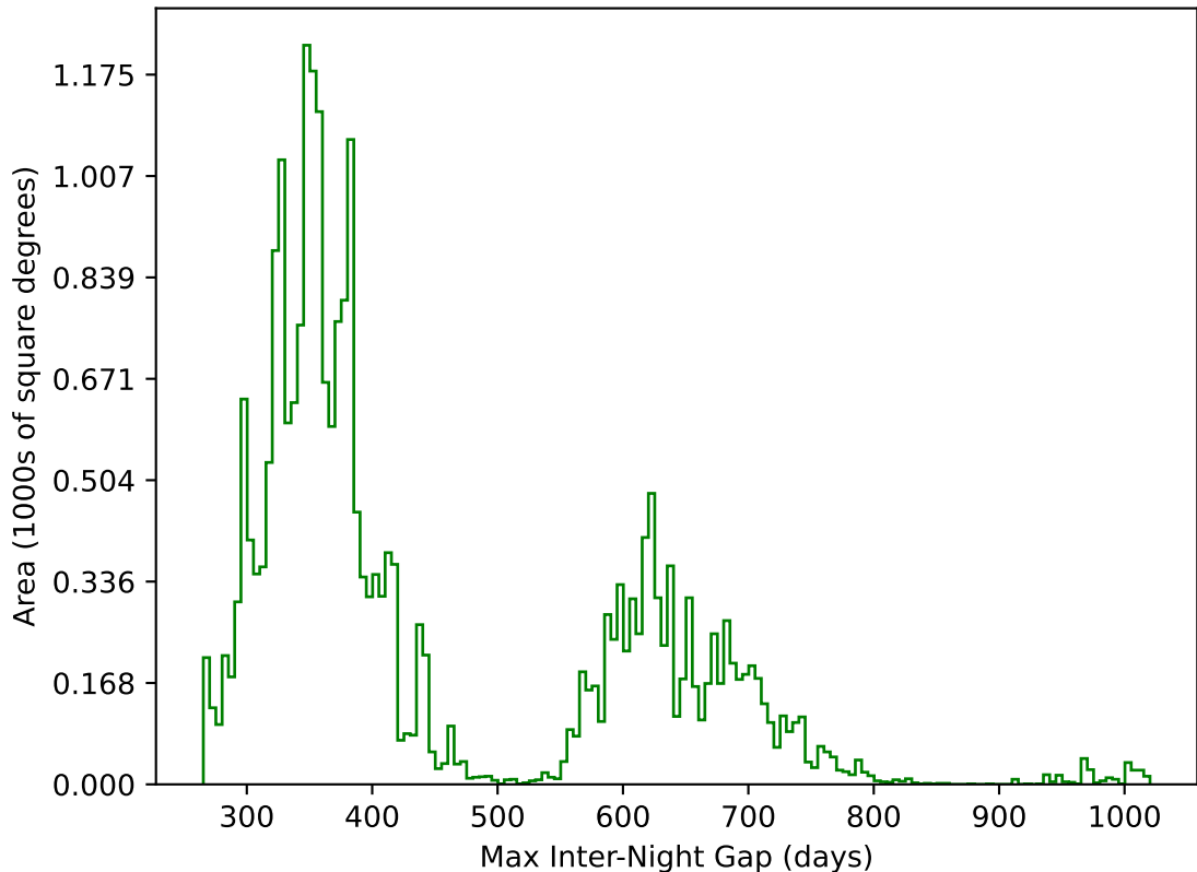
weather_cloudso0v3.4_10yrs All sky g band: Max Inter-Night Gap
