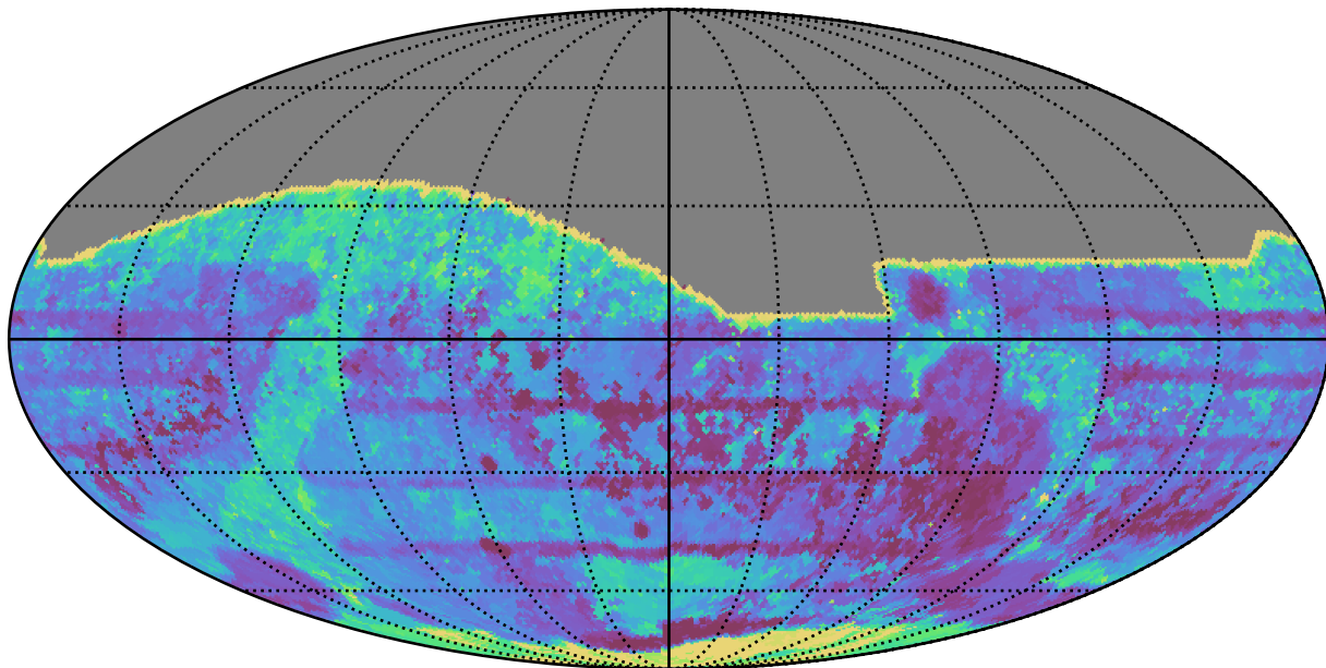
weather_cloudso0v3.4_10yrs All sky all bands: Max Inter-Night Gap
