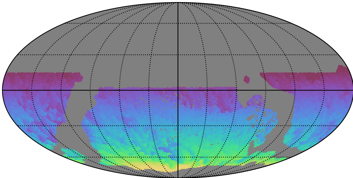
weather_cloudso0v3.4_10yrs WFD all bands: Max HA
