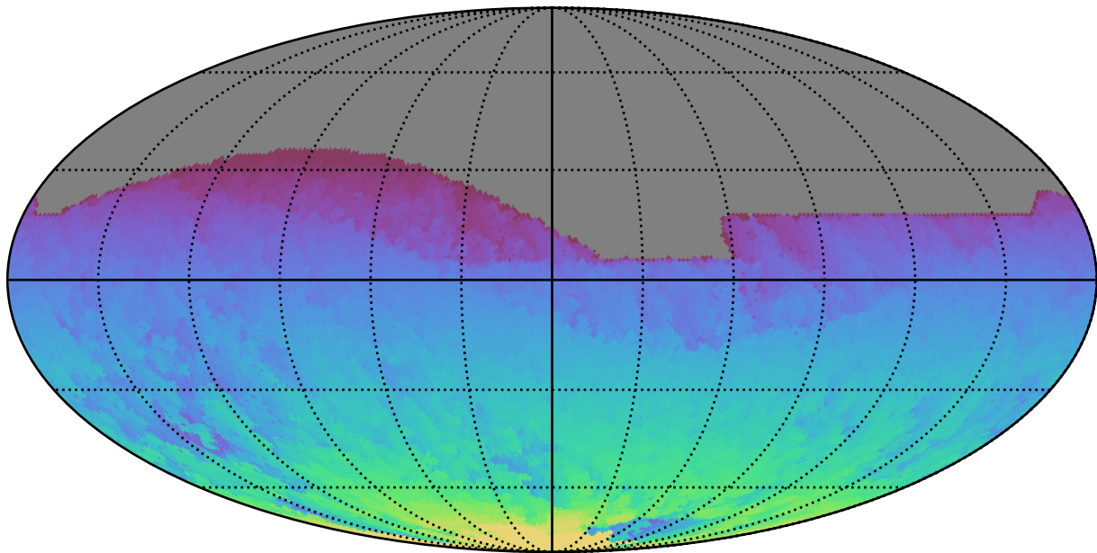
weather_cloudso0v3.4_10yrs All sky all bands: Max HA
