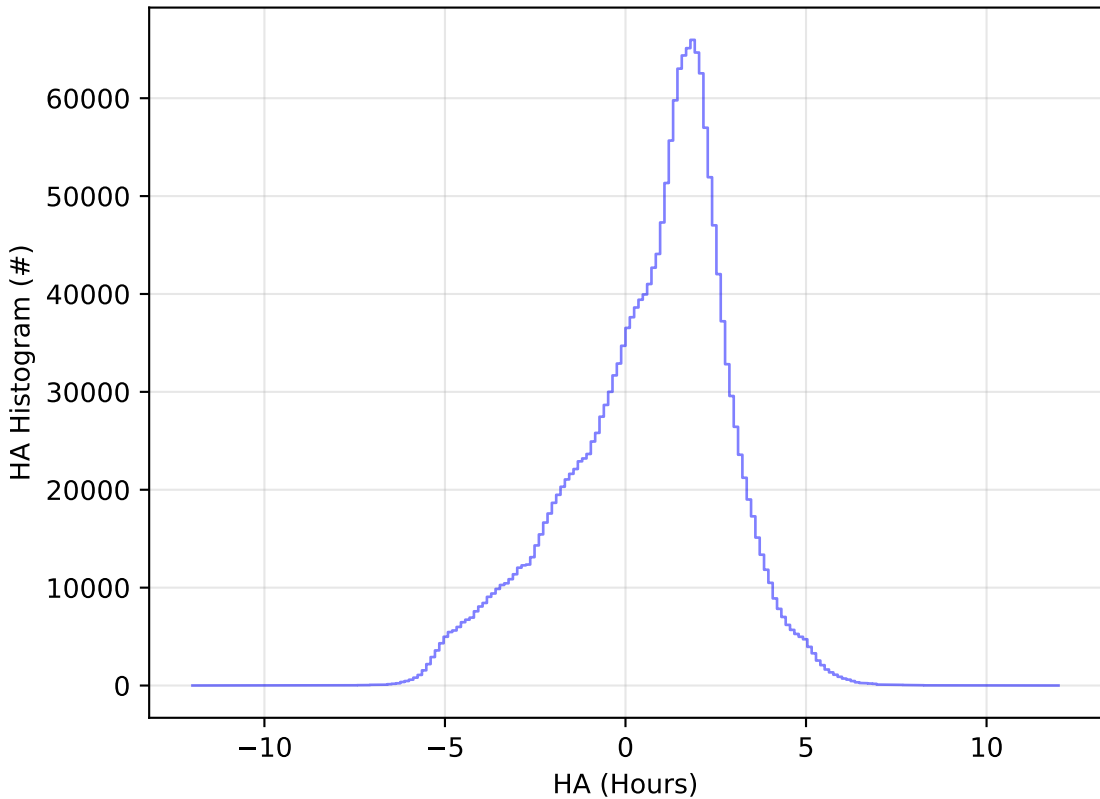
weather_cloudso0v3.4_10yrs WFD all bands: HA Histogram
