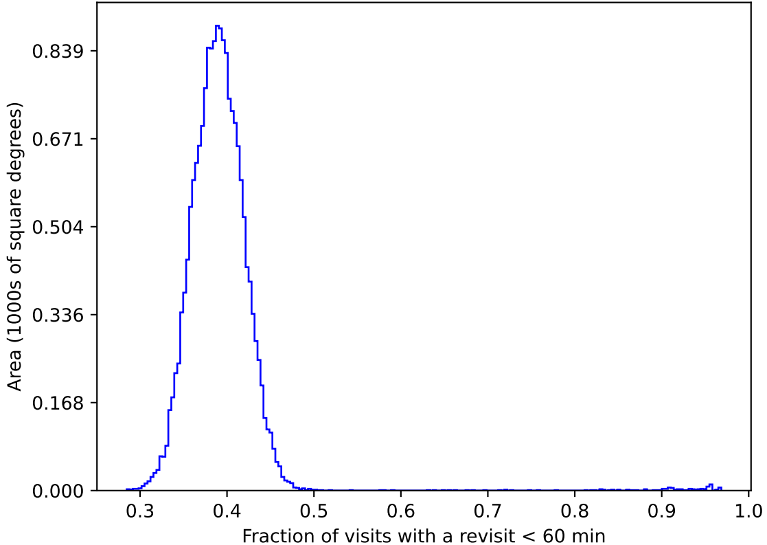
weather_cloudso0v3.4_10yrs gri WFD: Fraction of visits with a revisit < 60 min
