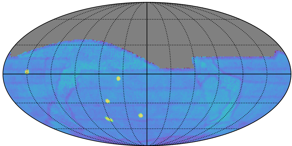
weather_cloudso0v3.4_10yrs gri All sky: Fraction of visits with a revisit < 60 min
