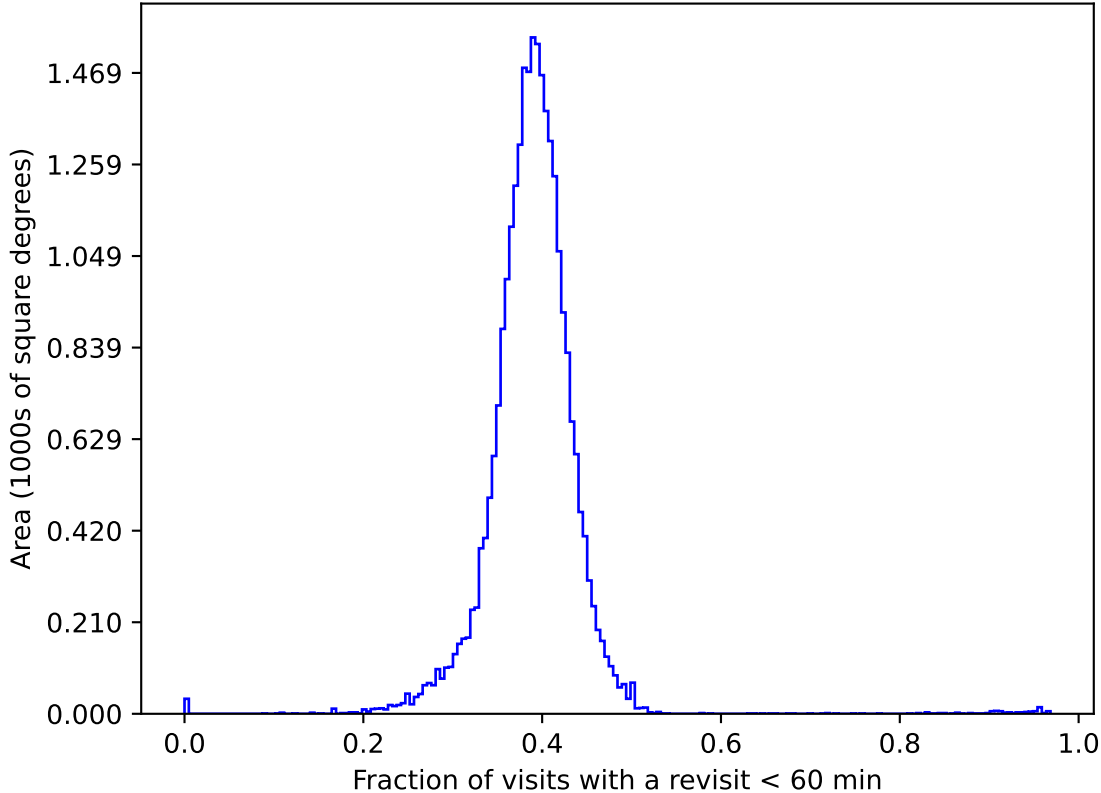
weather_cloudso0v3.4_10yrs gri All sky: Fraction of visits with a revisit < 60 min
