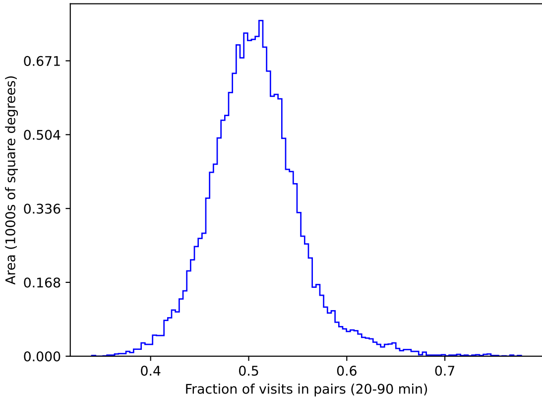
weather_cloudso0v3.4_10yrs gri WFD: Fraction of visits in pairs (20-90 min)
