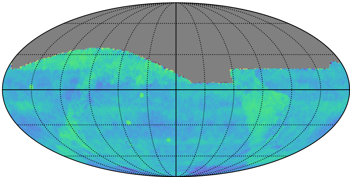
weather_cloudso0v3.4_10yrs gri All sky: Fraction of visits in pairs (20-90 min)
