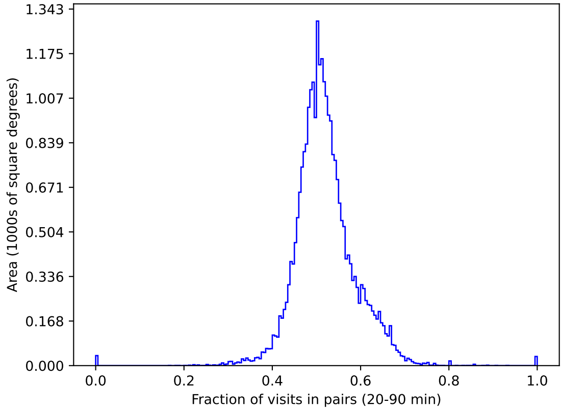
weather_cloudso0v3.4_10yrs gri All sky: Fraction of visits in pairs (20-90 min)
