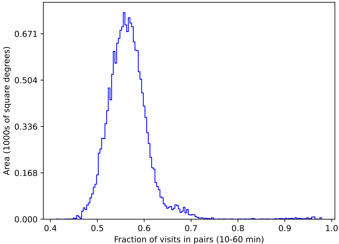
weather_cloudso0v3.4_10yrs gri WFD: Fraction of visits in pairs (10-60 min)
