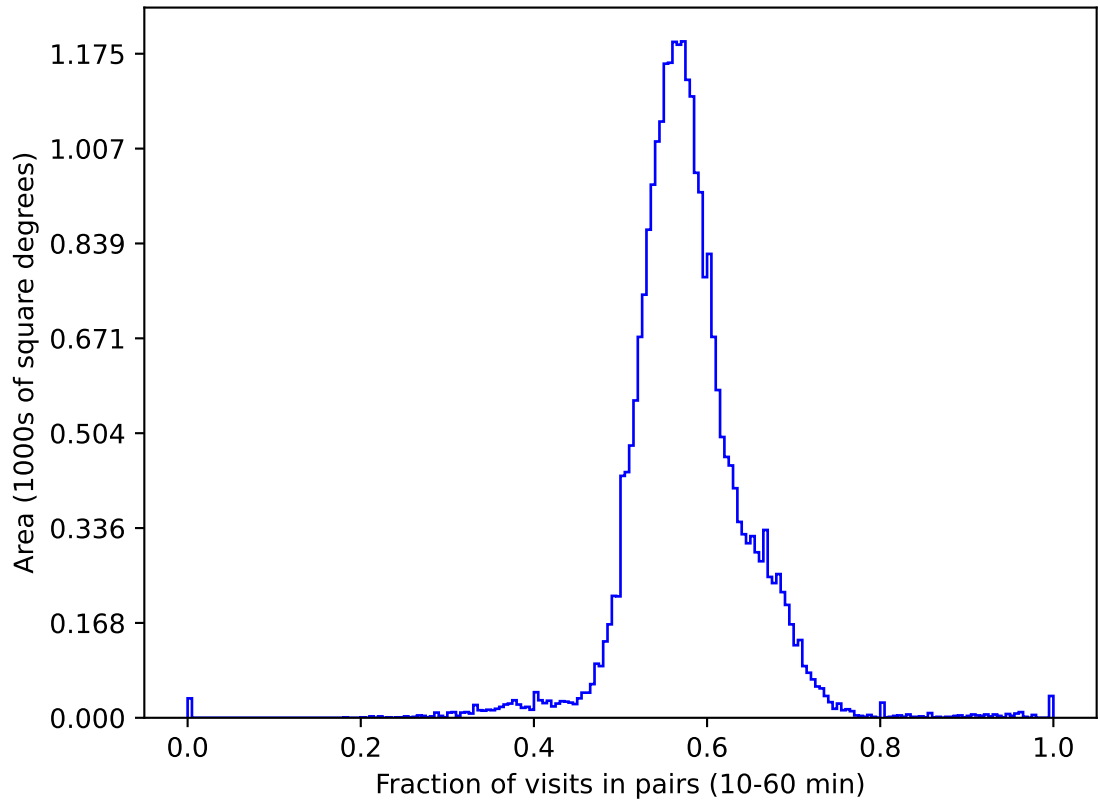
weather_cloudso0v3.4_10yrs gri All sky: Fraction of visits in pairs (10-60 min)
