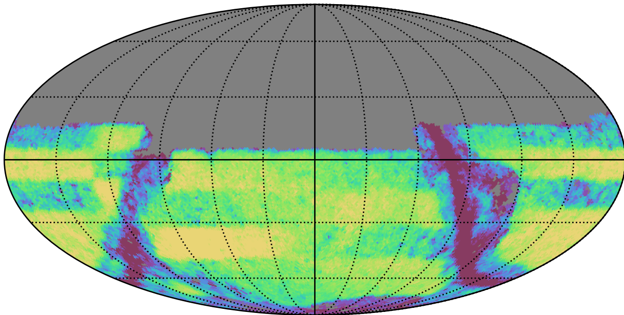
weather_cloudso0v3.4_10yrs Yr 3-4 y band: Exgal_CoaddM5
