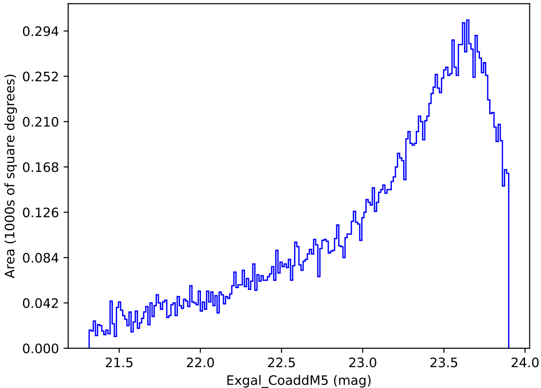
weather_cloudso0v3.4_10yrs Yr 3-4 y band: Exgal_CoaddM5
