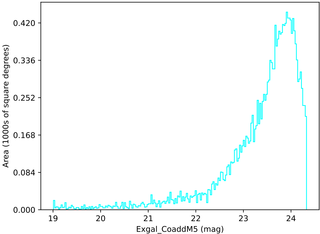
weather_cloudso0v3.4_10yrs Yr 3-4 u band: Exgal_CoaddM5
