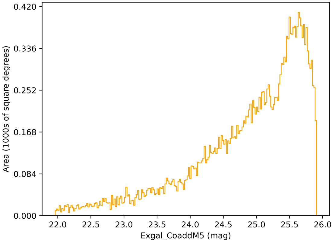
weather_cloudso0v3.4_10yrs Yr 3-4 r band: Exgal_CoaddM5
