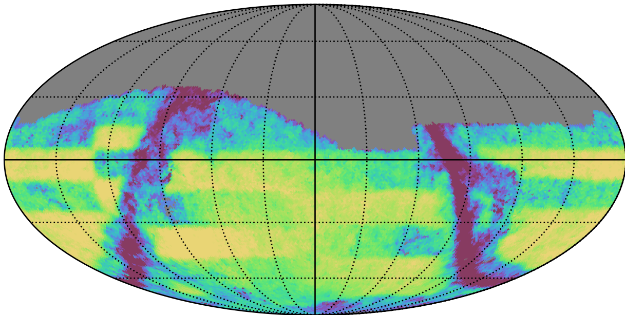
weather_cloudso0v3.4_10yrs Yr 3-4 i band: Exgal_CoaddM5
