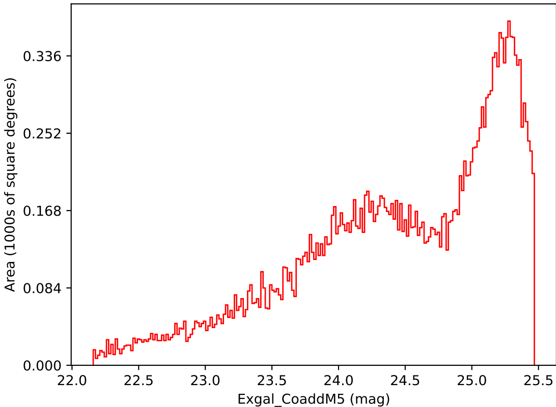
weather_cloudso0v3.4_10yrs Yr 3-4 i band: Exgal_CoaddM5
