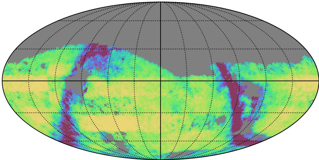
weather_cloudso0v3.4_10yrs Yr 3-4 g band: Exgal_CoaddM5
