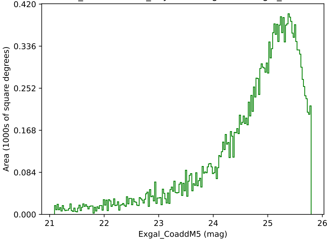
weather_cloudso0v3.4_10yrs Yr 3-4 g band: Exgal_CoaddM5
