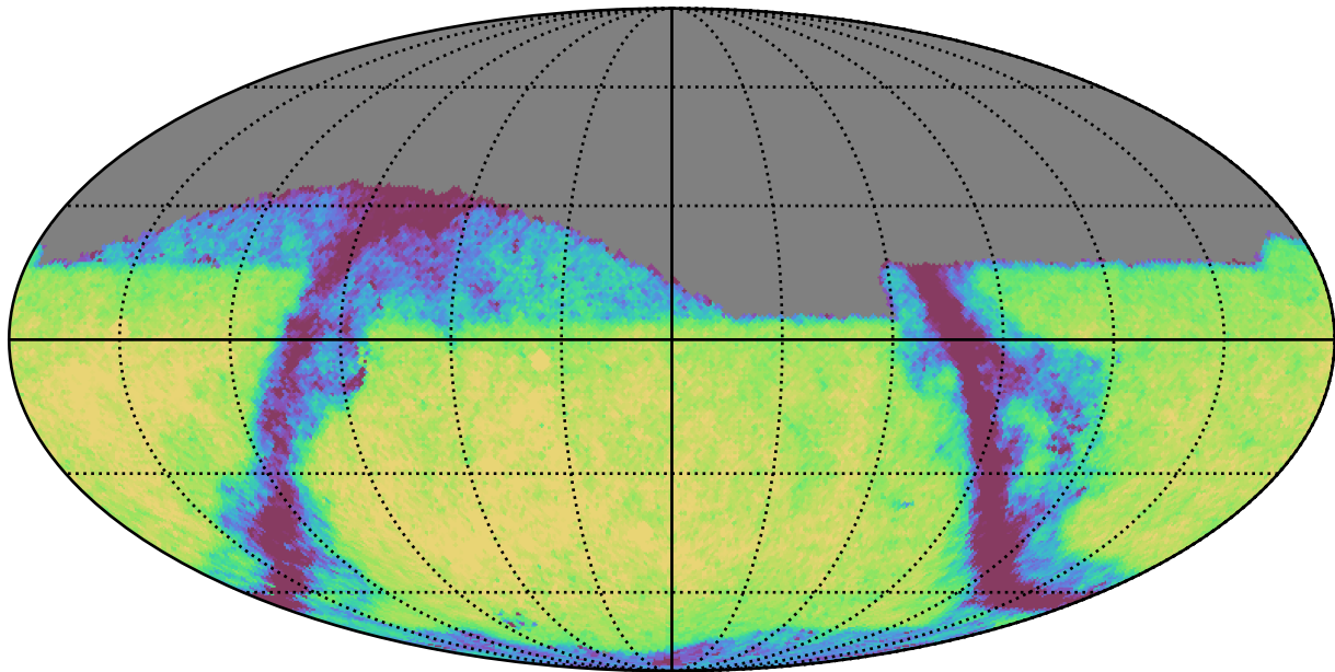
weather_cloudso0v3.4_10yrs Yr 1 z band: Exgal_CoaddM5
