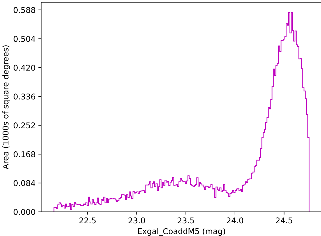
weather_cloudso0v3.4_10yrs Yr 1 z band: Exgal_CoaddM5
