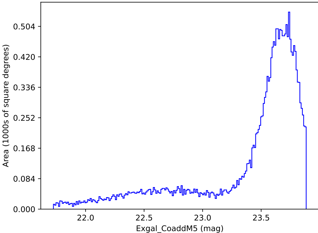
weather_cloudso0v3.4_10yrs Yr 1 y band: Exgal_CoaddM5
