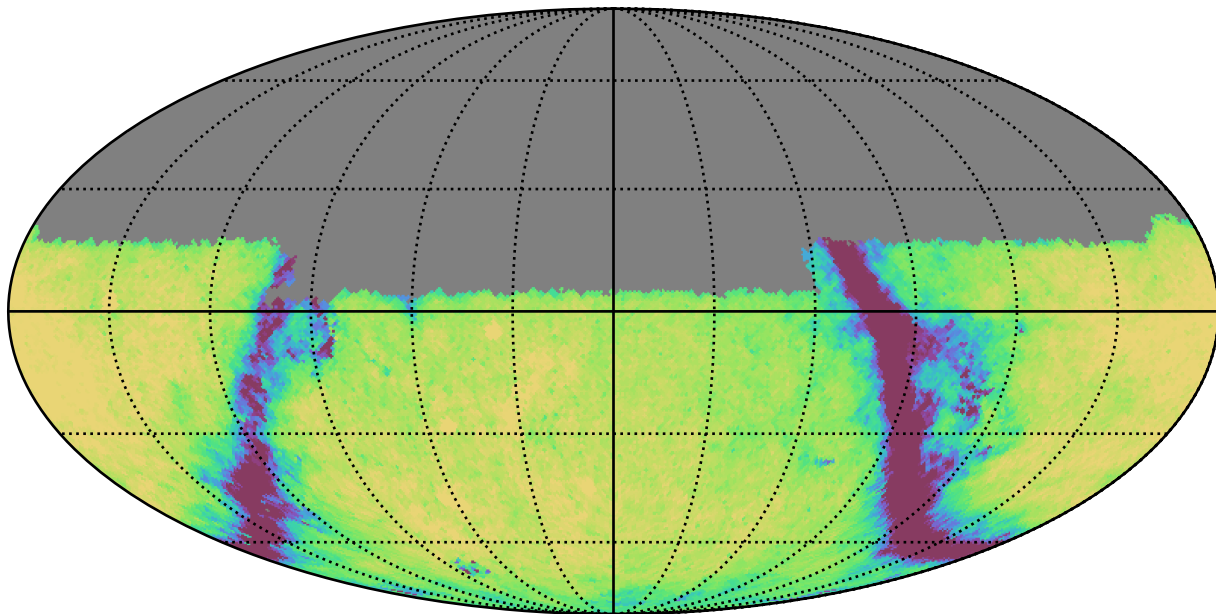
weather_cloudso0v3.4_10yrs Yr 1 u band: Exgal_CoaddM5
