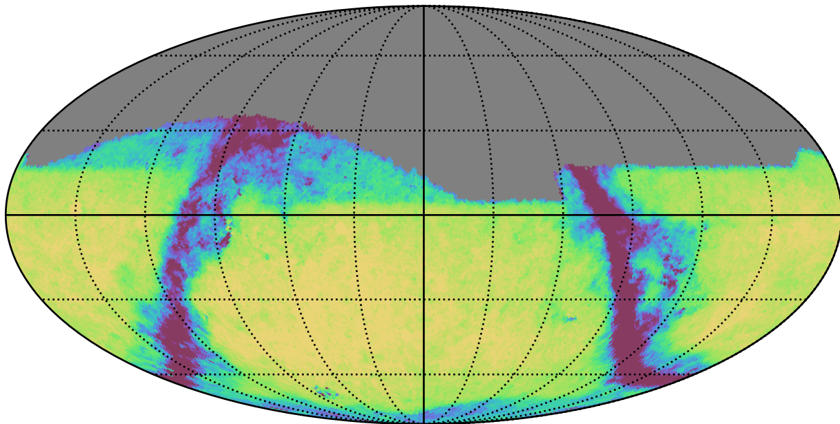
weather_cloudso0v3.4_10yrs Yr 1 r band: Exgal_CoaddM5
