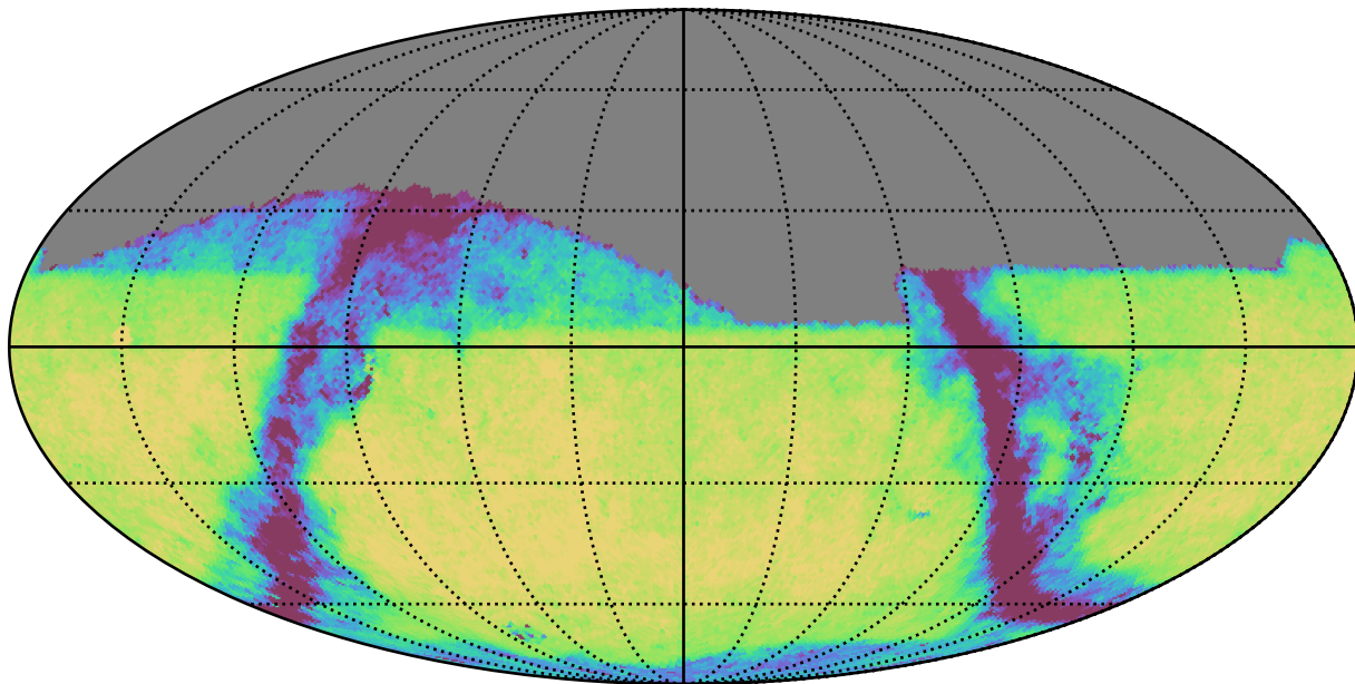
weather_cloudso0v3.4_10yrs Yr 1 i band: Exgal_CoaddM5
