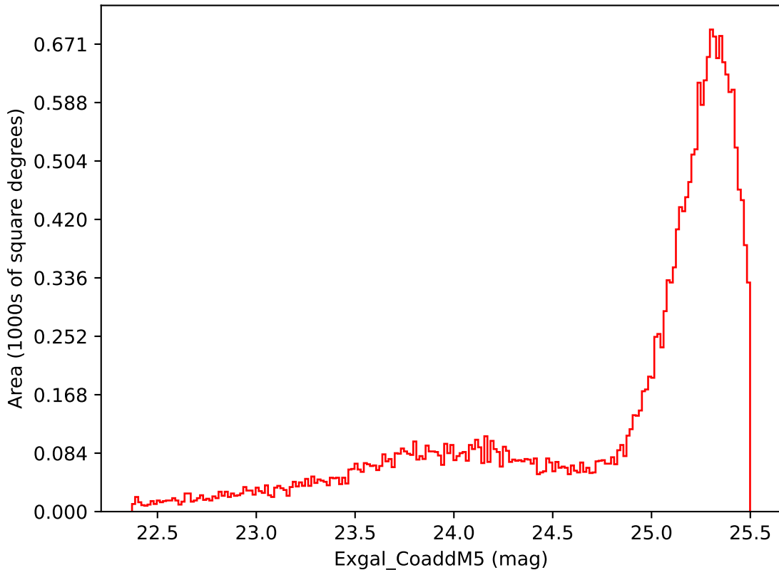
weather_cloudso0v3.4_10yrs Yr 1 i band: Exgal_CoaddM5
