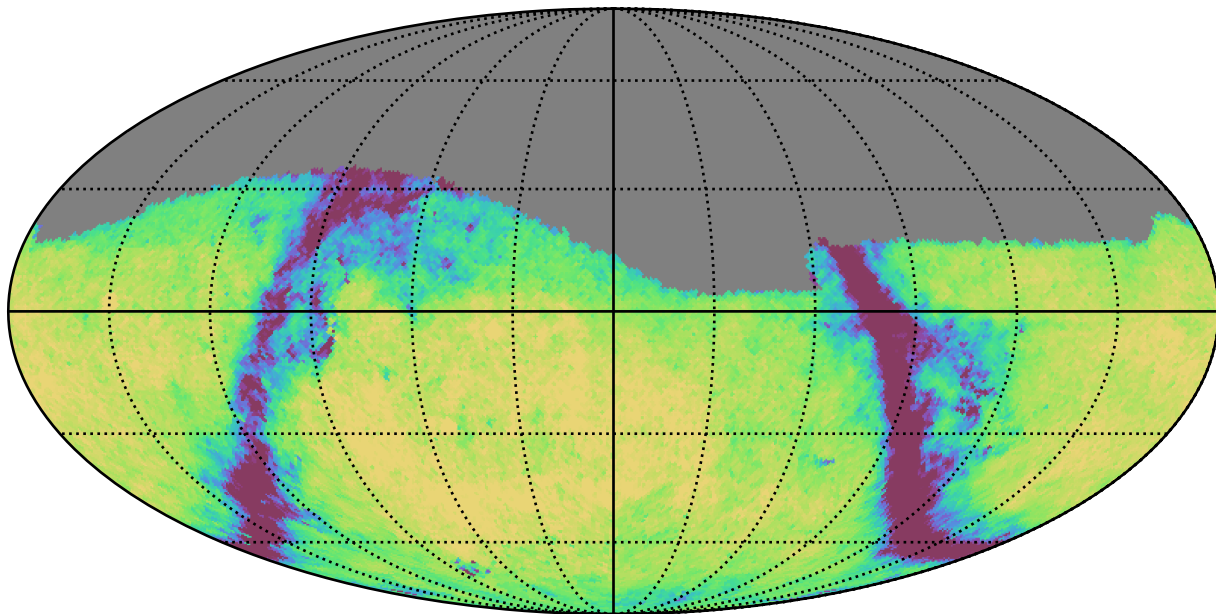
weather_cloudso0v3.4_10yrs Yr 1 g band: Exgal_CoaddM5
