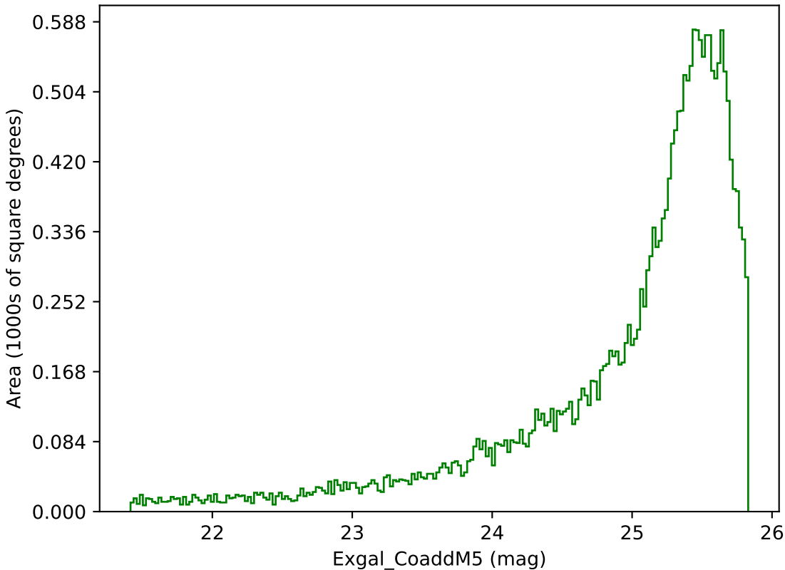
weather_cloudso0v3.4_10yrs Yr 1 g band: Exgal_CoaddM5
