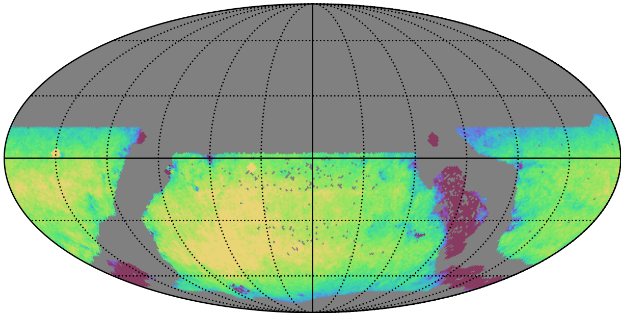
weather_cloudso0v3.4_10yrs WFD z band: Exgal_CoaddM5
